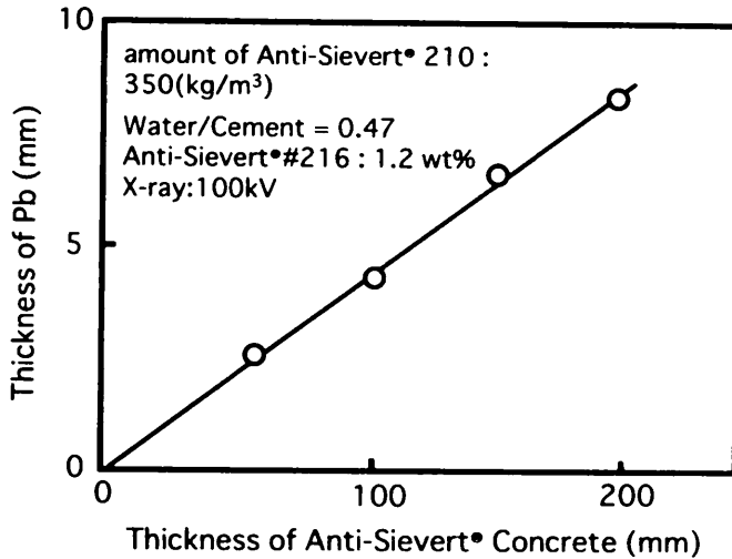
Figure 5 Relation of thickens of the Anti-Sievert concrete and thickness of Pb
