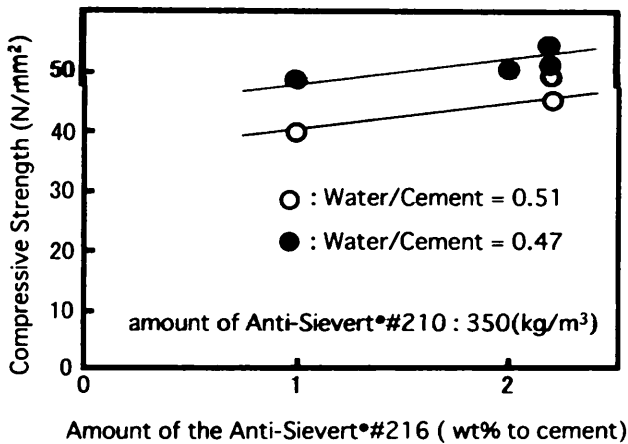
Figure 2 Compressive strength of the several Anti Sievert* concretes.
